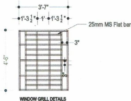
WINDOW GRILL DETAILS
