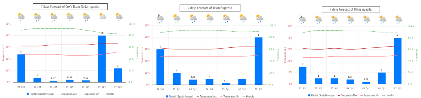
Figure 2: Daily rainfall average forecast.
