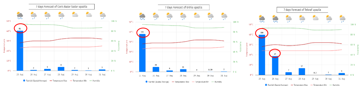
Figure 2: Daily rainfall average forecast.
