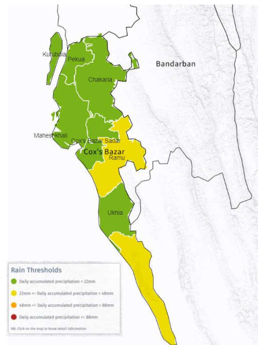
Figure 1: Seven days daily rainfall forecast threshold.
